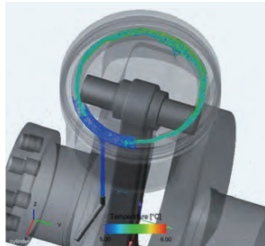
Piston cooling
