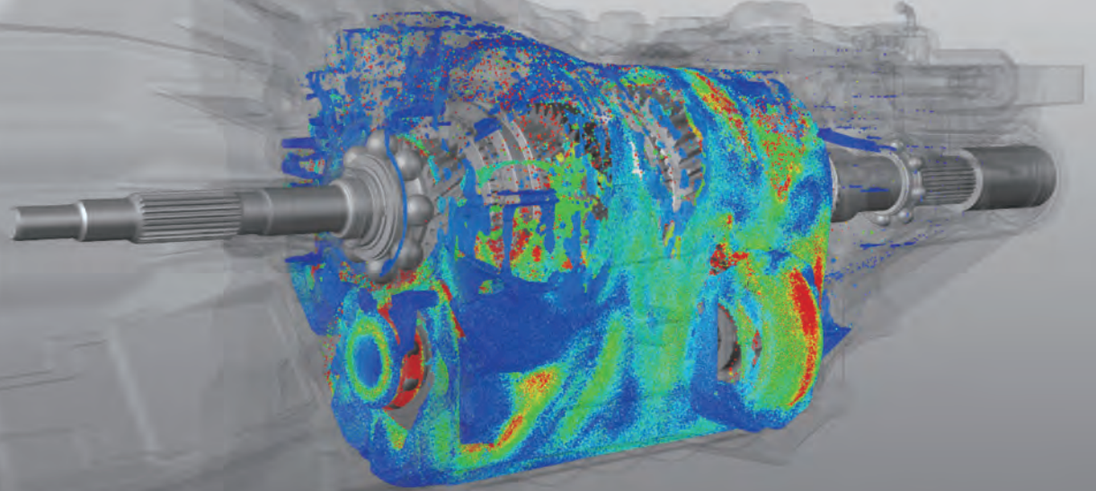
Oil distribution calculation in transmission Courtesy of UNIVANCE CORPORATION
