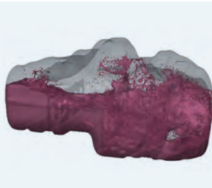
Fuel tank sloshing
